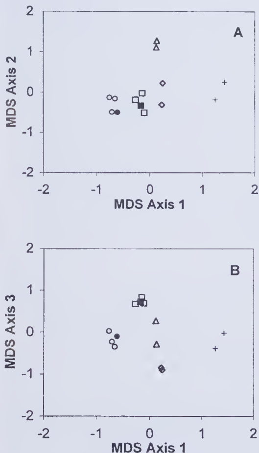
Figure 8. Three-dimensional ordination of invertebrate replicates and composite samples from Toolibin ( \square ) and Walbyring ( \circ ) Lakes, Lake Chandala ( \diamond ), Lake Cooloongup ( \Delta ), and 2 samples from a small wetland near Gingin (+) for different years (see text for details), showing discrimination between wetlands and proximity of replicates to the composite samples (filled symbols); stress = 0.09.
